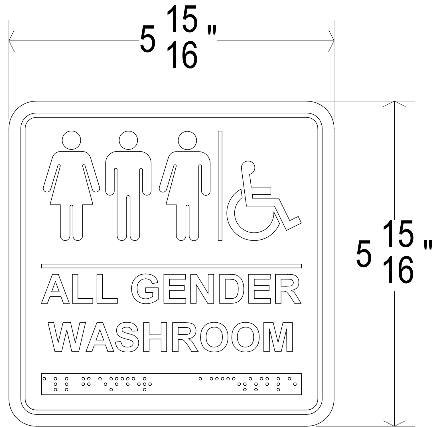
Front view
