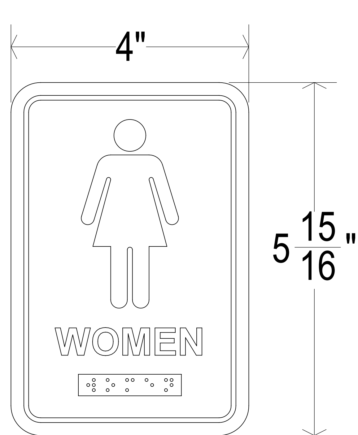
Front view
