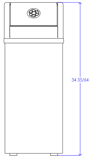
Front View 301R NL
