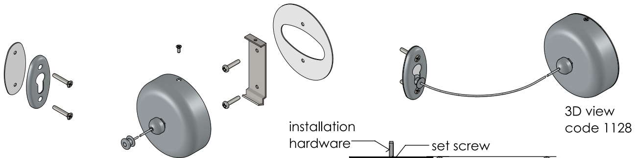
3D view -assembly
